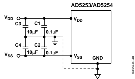
Figure 40. Power Supply Bypassing
